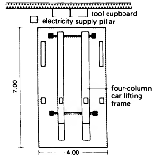
③ Optical alignment checking 4.0m x 7.0m
